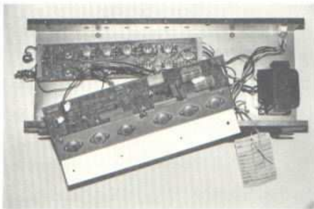
Pre-amp Disassembly – Diagram Three
