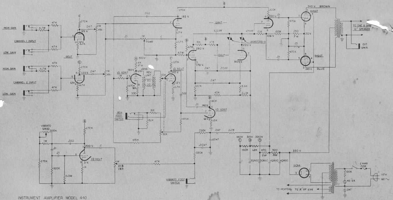
INSTRUMENT AMPLIFIER MODEL 440 117 VOLTS 60 CYCLES 100 WATTS MANUFACTURED BY ESTEY ELECTRONIC INC. TORRANCE, CALIFORNIA
