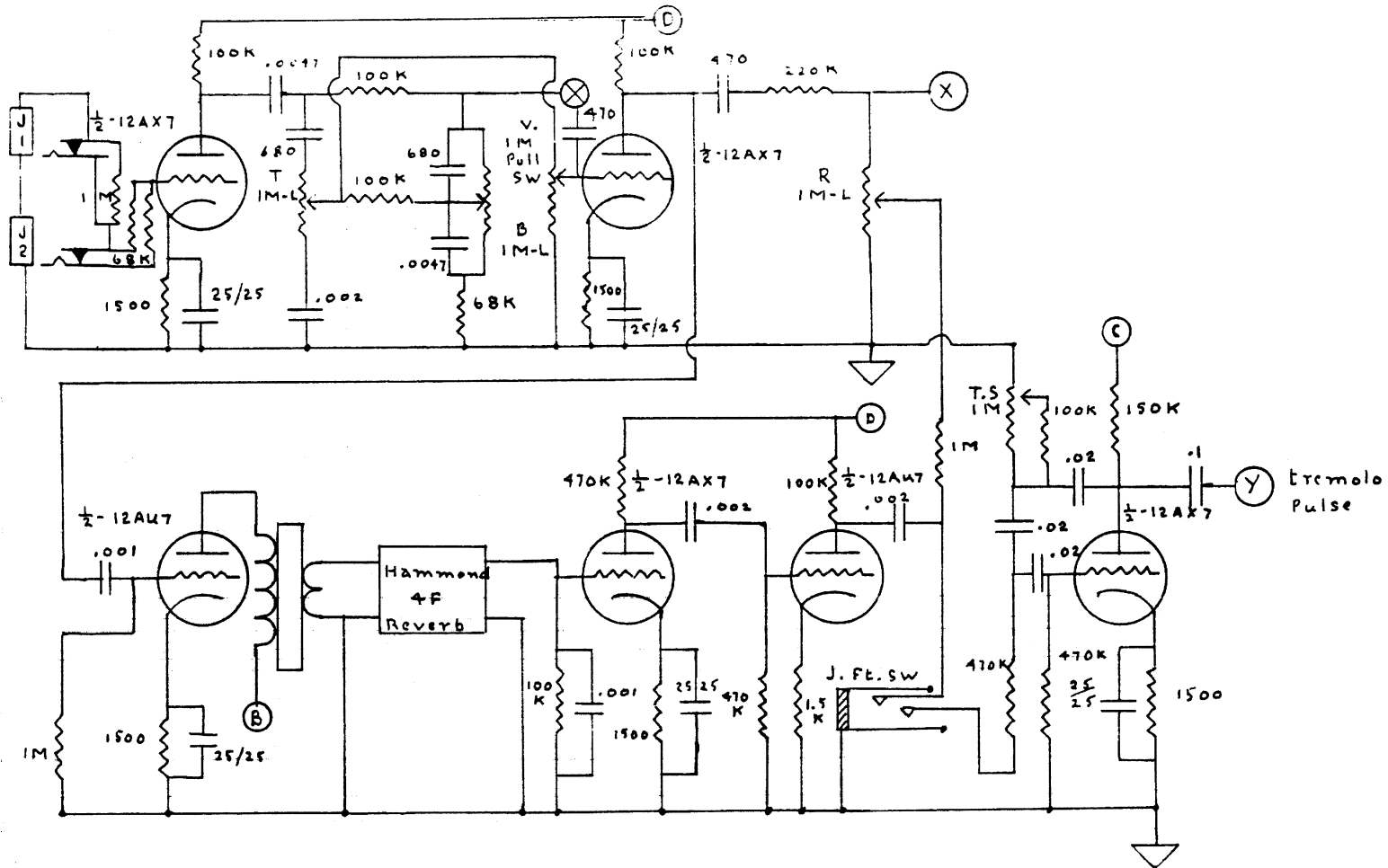
Pre-amp - Reverb and tremolo for G45TR, G90TR, G100TR, LB100TR
