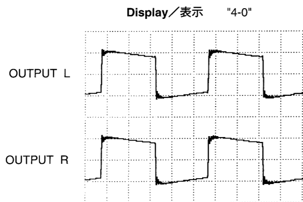
Fig.3/図3 (1mS/DIV, 0.1V/DIV)
