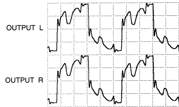
Fig.5/図5 (1mS/DIV, 0.2V/DIV)
