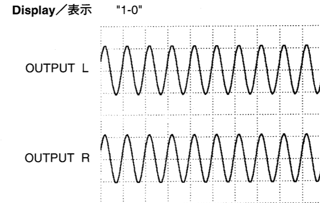
Fig.2/図2 (1mS/DIV, 0.1V/DIV)
