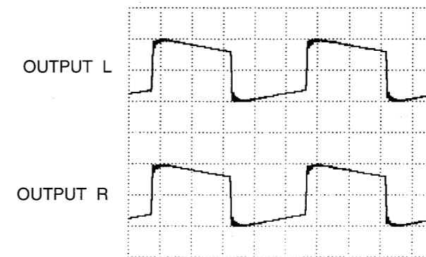
Fig4/図4 (1mS/DIV, 0.1V/DIV)
