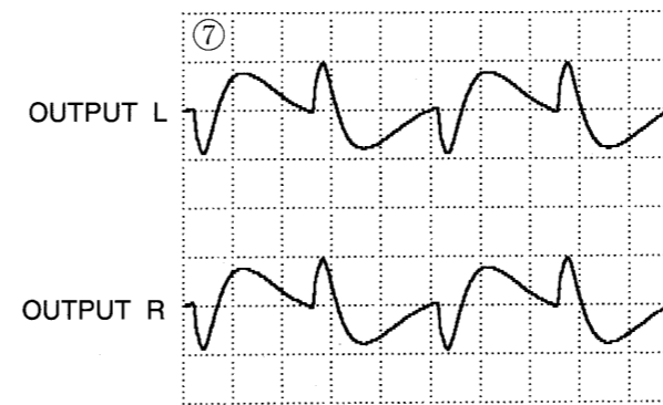
Fig.6/図6 (1mS/DIV, 0.2V/DIV)
