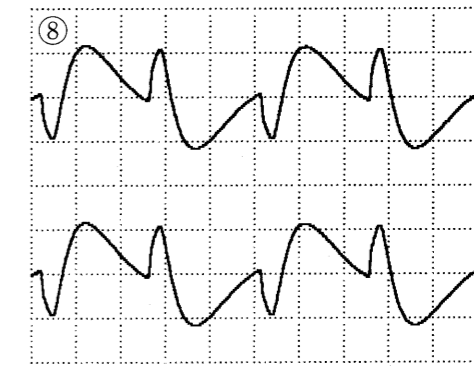
Fig.6/図6 (1mS/DIV, 0.2V/DIV)
